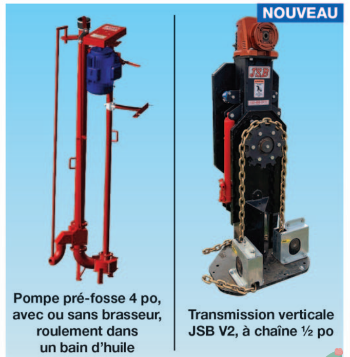
Transmission rehaussée
